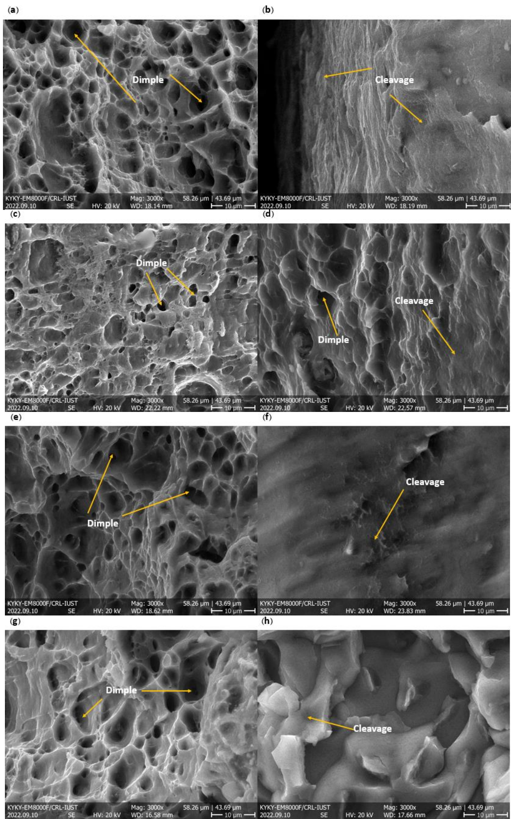
Fig. 14. SEM images from the fracture surfaces, a) 2-layer Al section- room temperature, b) 2-layer Mg section- room temperature, c) 2-layer Al section-200°C, d) 2-layer Mg section-200°C, e) 2-layer Al section-300°C, f) 2-layer Mg section-300°C, g) 2-layer Al section-400°C, h) 2-layer Mg section-400°C
