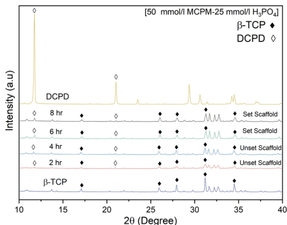
Fig. 2. The XRD peaks of unset and set porous DCPD/β-TCP scaffolds after exposure the 300-600 μm of porous β-TCP granules with 50 mmol/l concentrations of acidic-CaP solution at four different setting-time reactions [2, 4, 6, and 8 hours].
