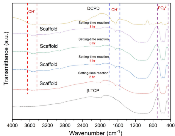
Fig. 3. The FTIR results of porous DCPD/β-TCP scaffolds after exposing 300-600 μm of porous β-TCP granules to 50 mmol/l of acidic-CaP solution at four different setting reaction times [2, 4, 6, and 8 hours].
