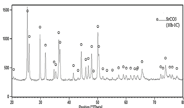
Fig. 7. XRD analysis of the final SrCO 3 precipitate of the sample 10h-1C
