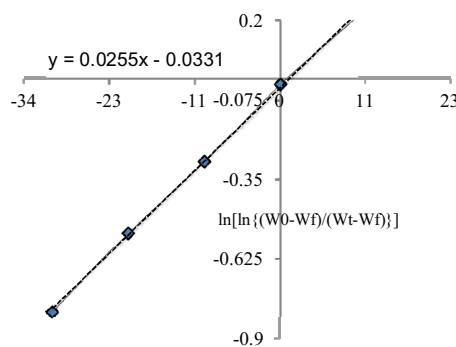
Fig. 6. Calculation of Energy of Activation for pure LS
