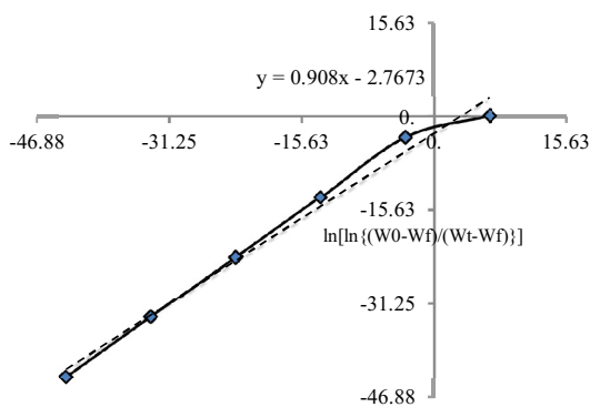
Fig. 5. Calculation of Energy of Activation for blend SA/LS (60/40).
